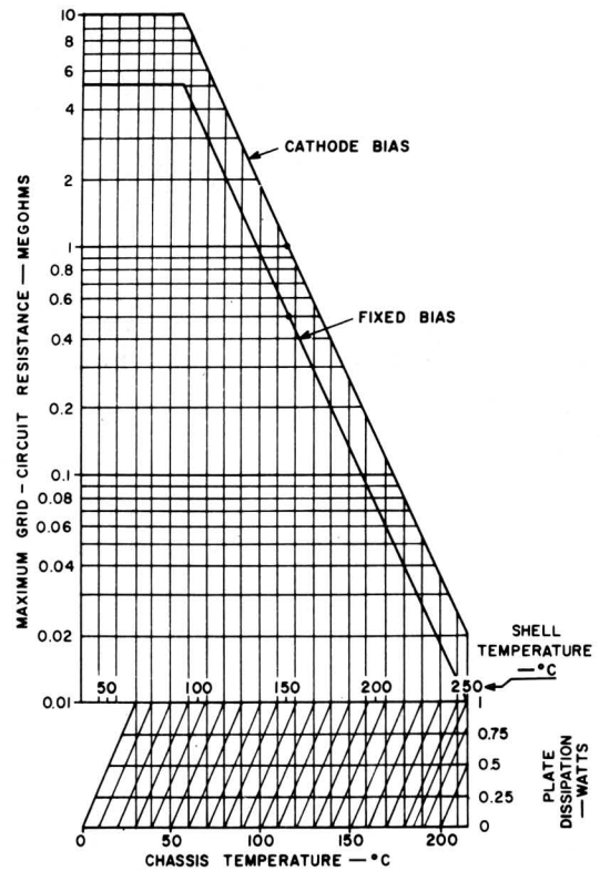
Fig. 11 - Nomograph for type 8058.
